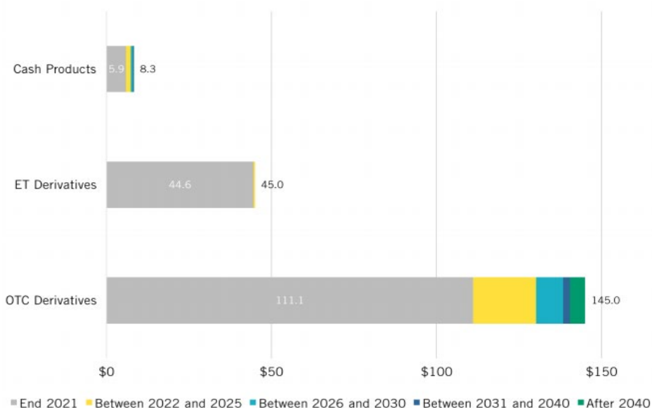
Fig 12 Gross notional of all financial product referencing dollar Libor (USDtrn)
